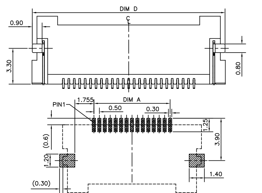
RECOMMENDED PCB LAYOUT(TOP VIEW) GENERAL TOLERANCE ±0.05
