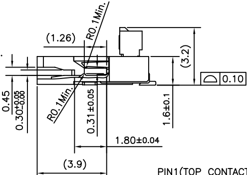
(ACTUATOR OPEN)
